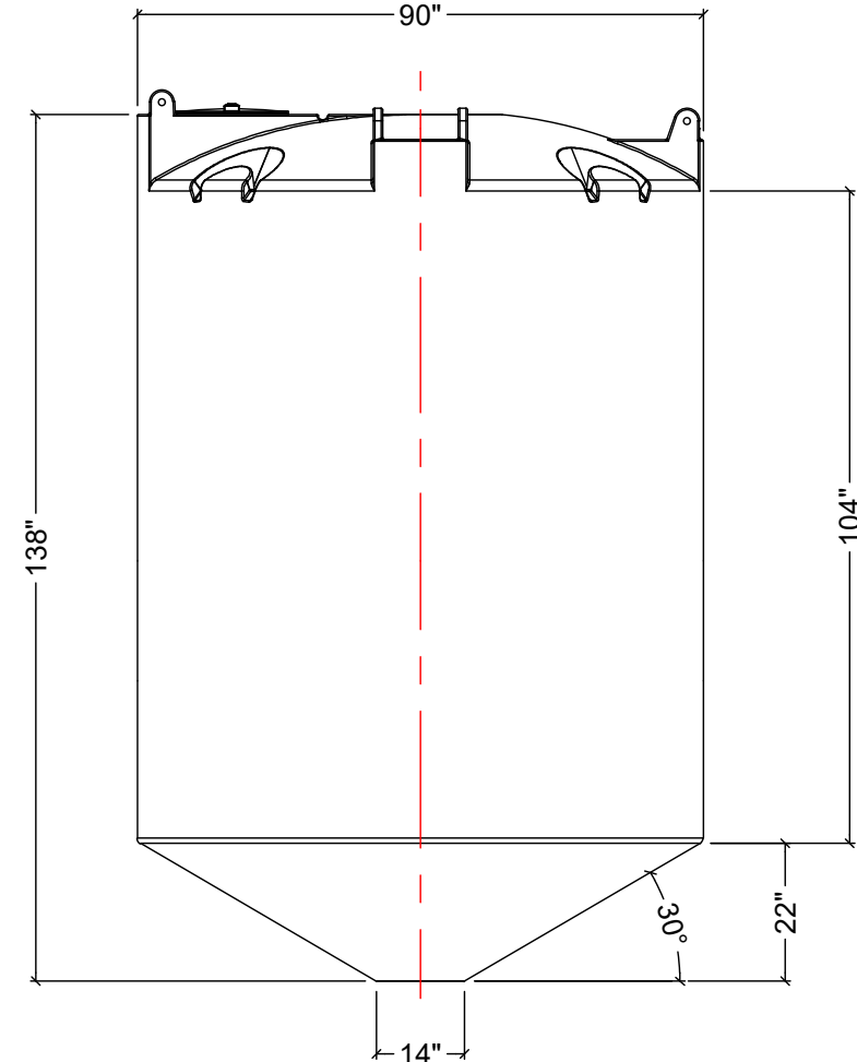
SIDE VIEW
